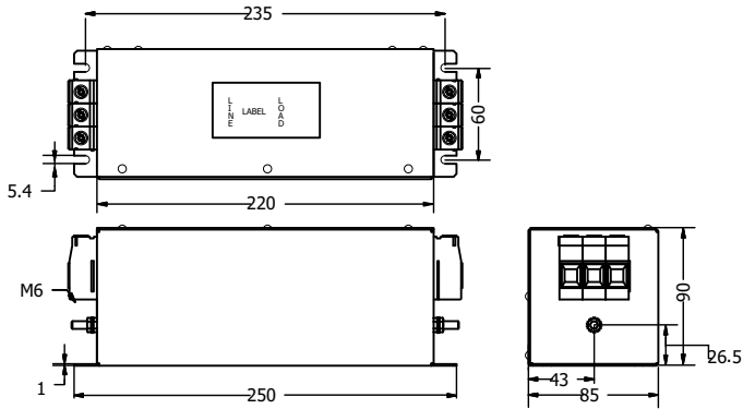
100 & 130Amp Terminal block (50mm 2 )
