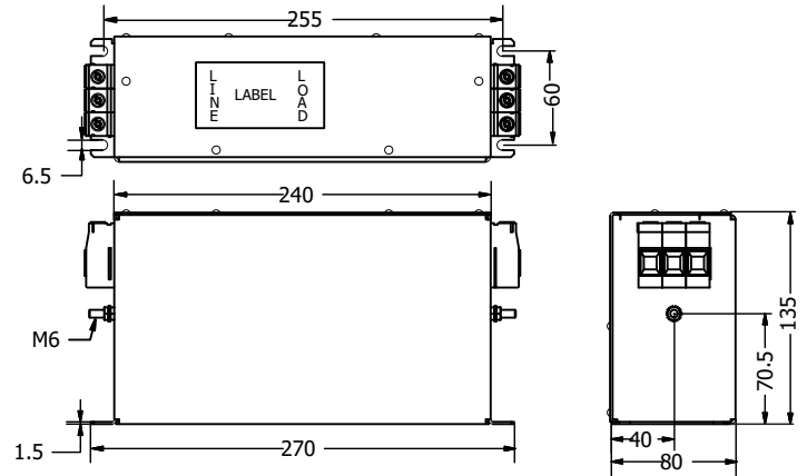
200Amp Terminal block (95mm 2 )
