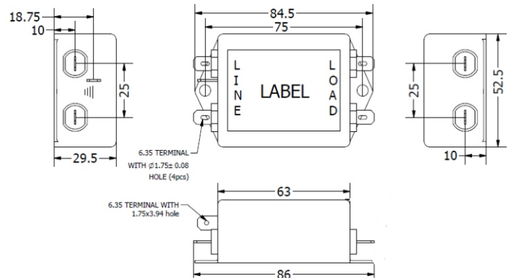
16 & 20 Amp Faston Terminal
