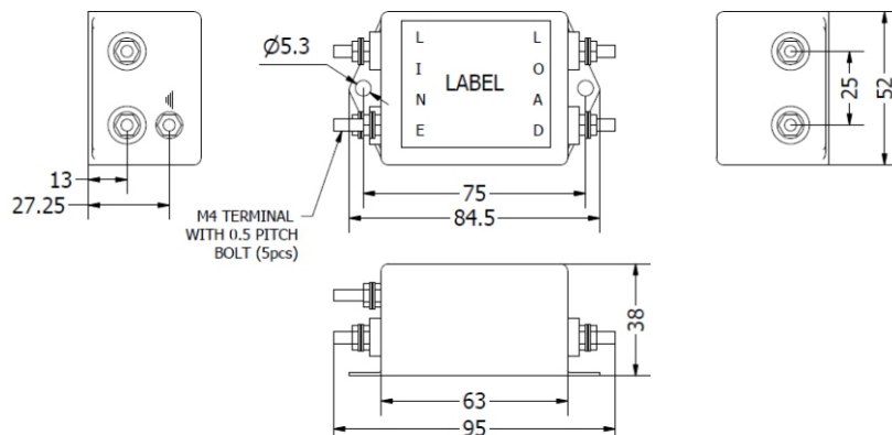
20 & 30 Amp Screw Terminal (M4)
